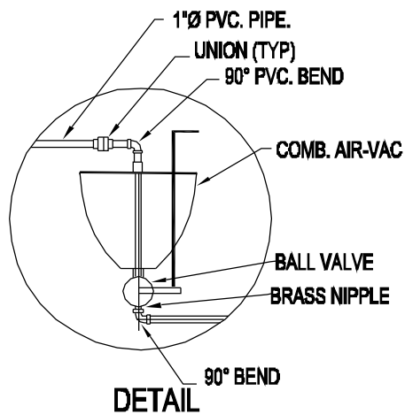
AIR RELEASE VALVE AND ROADWAY DETAIL
